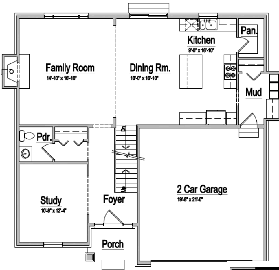
FIRST FLOOR 1,089 SQ. FT.
